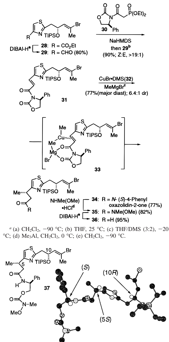
Figure 4. Structure of Weinreb amidation byproduct 37 and its X-ray crystal structure (Chem 3D representation). Hydrogen atoms are omitted, except at stereogenic centers, for clarity.
