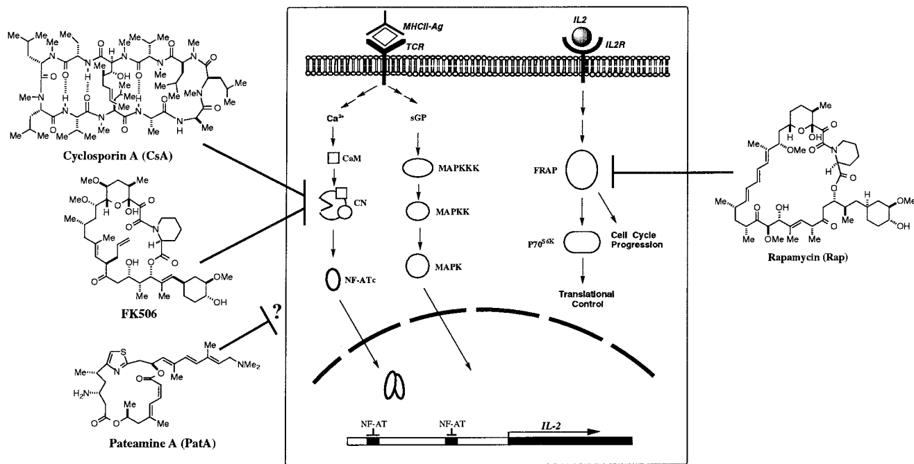
Figure 1. Signal transduction pathways involved in T lymphocyte activation and the site of action of the immunosuppressants cyclosporin A, FK506, rapamycin and pateamine A. Abbreviations: MHCII-Ag, major histocompatibility complex II–antigen complex; TCR, T cell receptor; IL2, interleukin 2; IL2R, the IL2 receptor; CaM, calmodulin; CN, calcineurin; NF-AT, nuclear factor of activated T cells; NF-ATc, the cytoplasmic subunit of NF-AT; FRAP, FKBP–rapamycin-associated protein; sGP, small GTP binding proteins; MAPK, generic MAP kinases; MAPKK, MAPK kinase; MAPKKK, MAPKK kinase.
